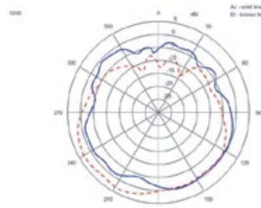
5 GHZ Peak Gain: 5.8 DBI
