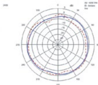
2.4 GHZ Peak Gain: 3.6 DBI
